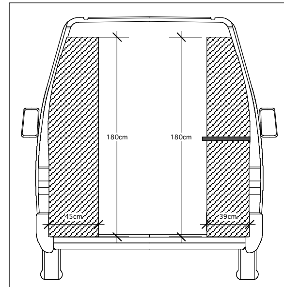
AGENCEMENT BOXER/DUCATO/JUMPER L2H2 (TRADE ADVANCE) VUE ARRIERE
