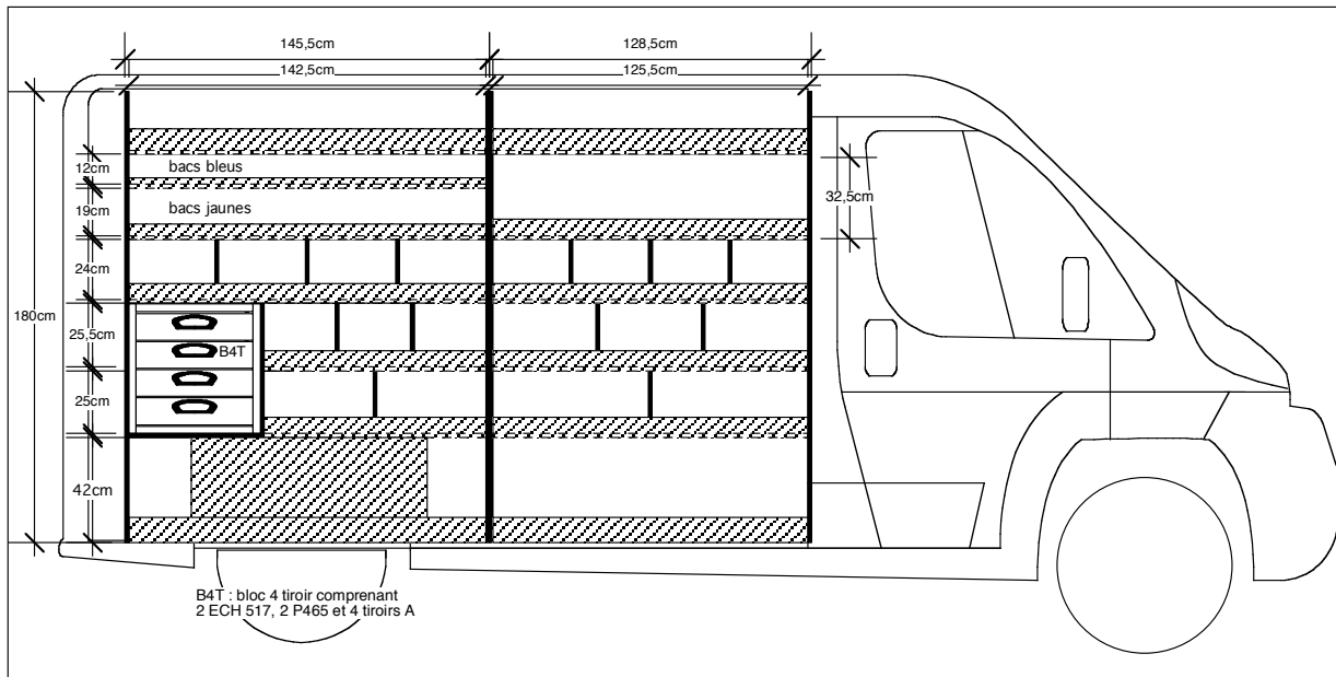
AGENCEMENT BOXER/DUCATO/JUMPER L2H2 (TRADE ADVANCE) VUE GAUCHE
