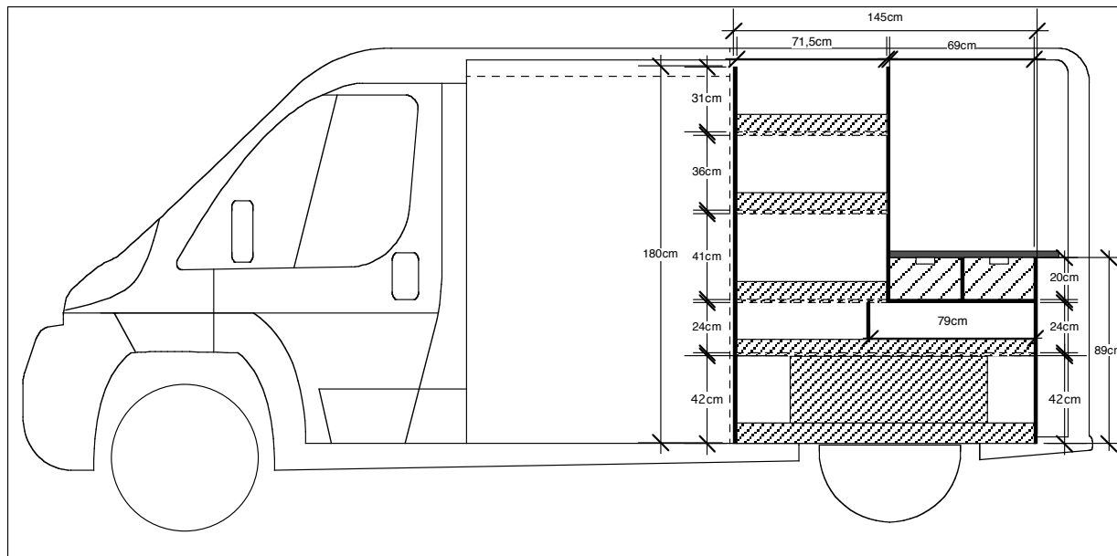
AGENCEMENT BOXER/DUCATO/JUMPER L2H2 (TRADE ADVANCE) VUE DROITE
