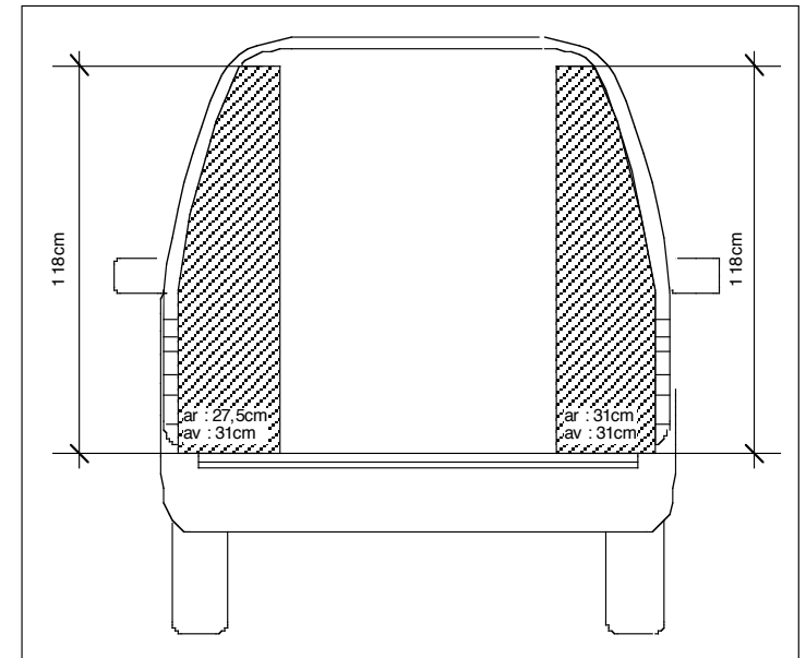
AGENCEMENT CADDY (TRADE ADVANCE) VUE ARRIERE
