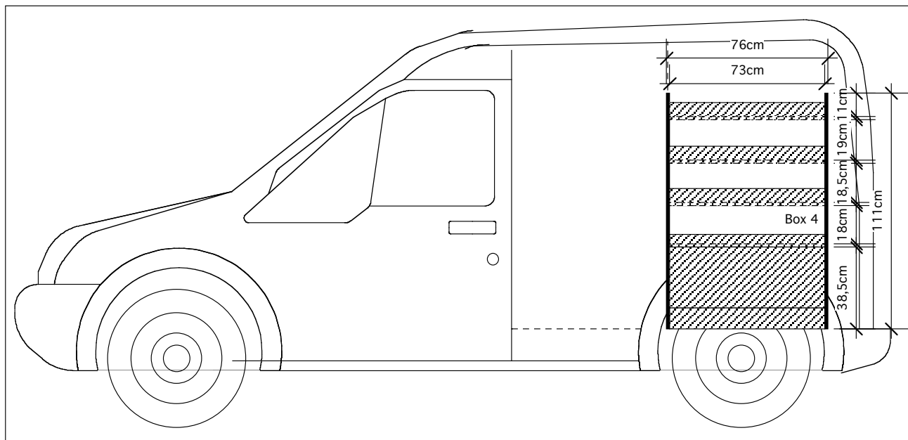
AGENCEMENT FORD CONNECT COURT (TRADE ADVANCE) VUE DROITE
