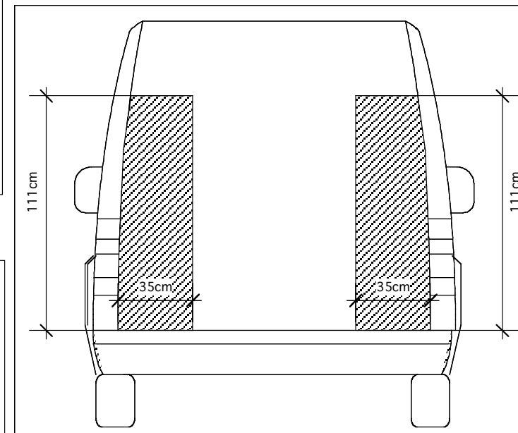
AGENCEMENT FORD CONNECT COURT (TRADE ADVANCE) VUE ARRIERE
