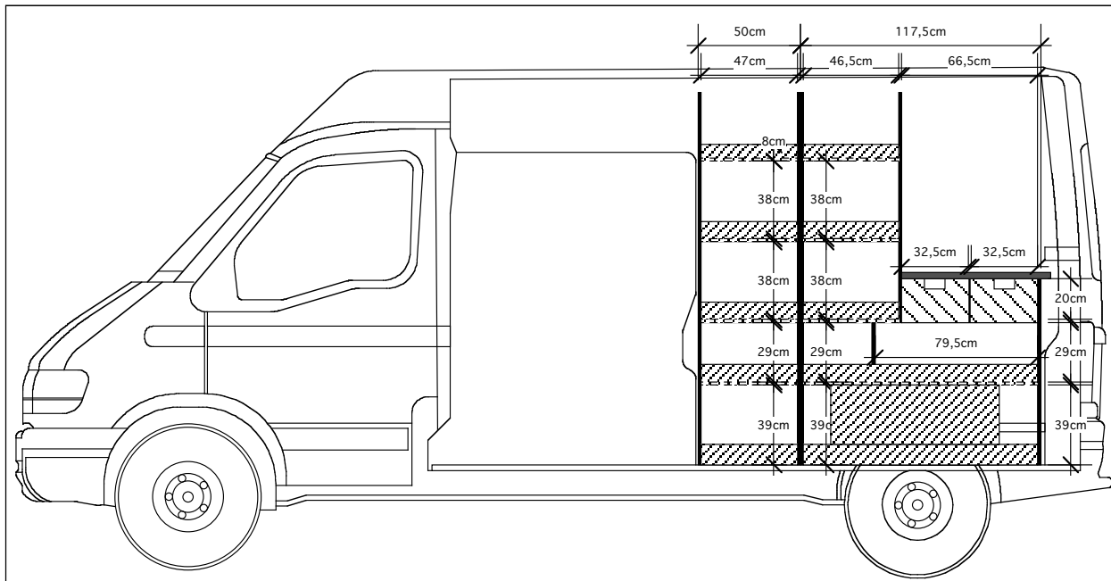
MASTER/MOVANO/INTERSTAR L2 (TRADE ADVANCE) VUE DROITE
