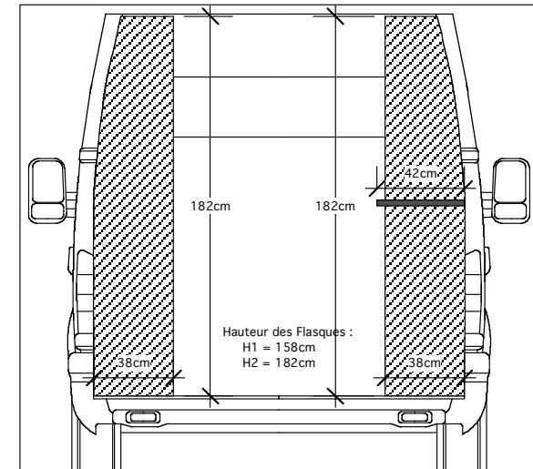
MASTER/MOVANO/INTERSTAR L2 (TRADE ADVANCE) VUE ARRIERE
