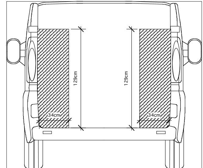
AGENCEMENT TRAFIC/VIVARO/PRIMASTAR L1H1 (TRADE ADVANCE) VUE ARRIERE
