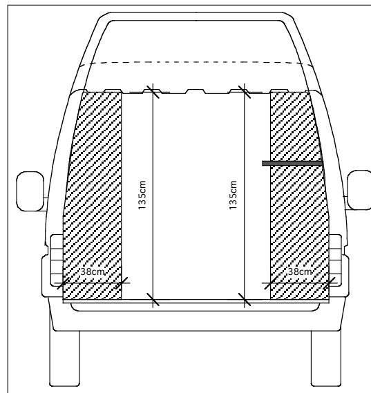
AGENCEMENT TRANSIT COURT BAS (TRADE ADVANCE) VUE ARRIERE
