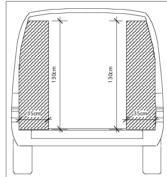
AGENCEMENT TRANSPORTER T5 COURT (TRADE ADVANCE) VUE ARRIERE
