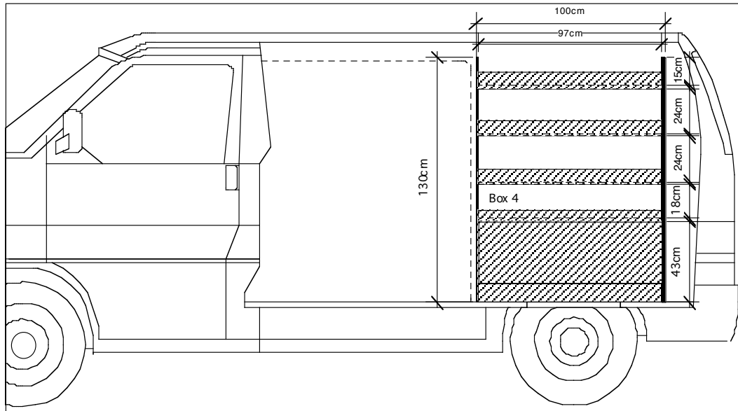
AGENCEMENT TRANSPORTER T5 COURT (TRADE ADVANCE) VUE DROITE
