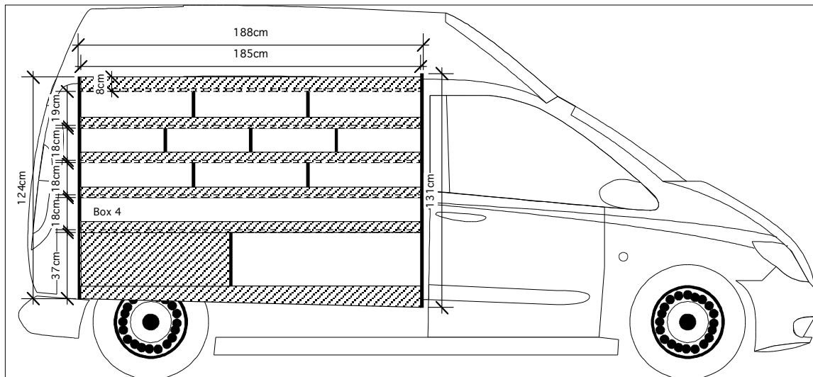
AGENCEMENT VITO COMPACT (TRADE ADVANCE) VUE GAUCHE
