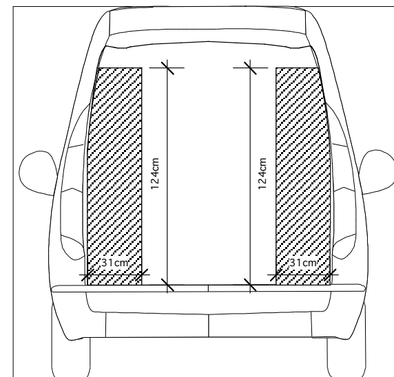
AGENCEMENT VITO COMPACT (TRADE ADVANCE) VUE ARRIERE
