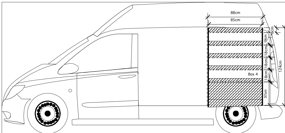
AGENCEMENT VITO COMPACT (TRADE ADVANCE) VUE DROITE
