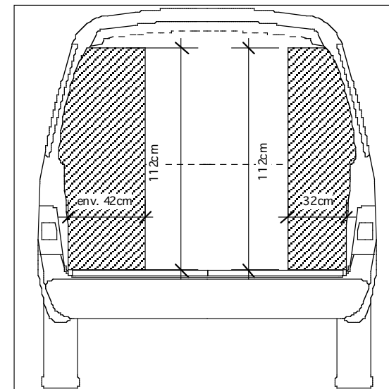
AGENCEMENT BERLINGO/PARTNER/KANGOO PL (TRADE ADVANCE) VUE ARRIERE
