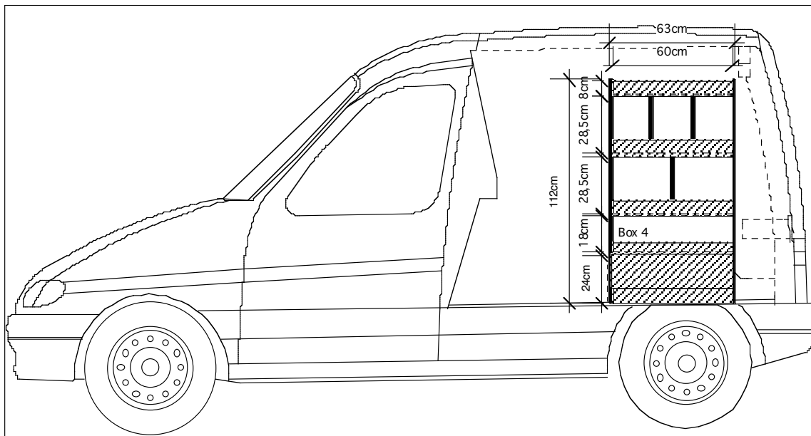
AGENCEMENT BERLINGO/PARTNER/KANGOO PL (TRADE ADVANCE) VUE DROITE
