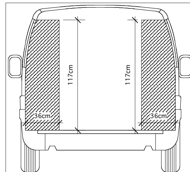
AGENCEMENT DOBLO COURT PL (TRADE ADVANCE) VUE ARRIERE
