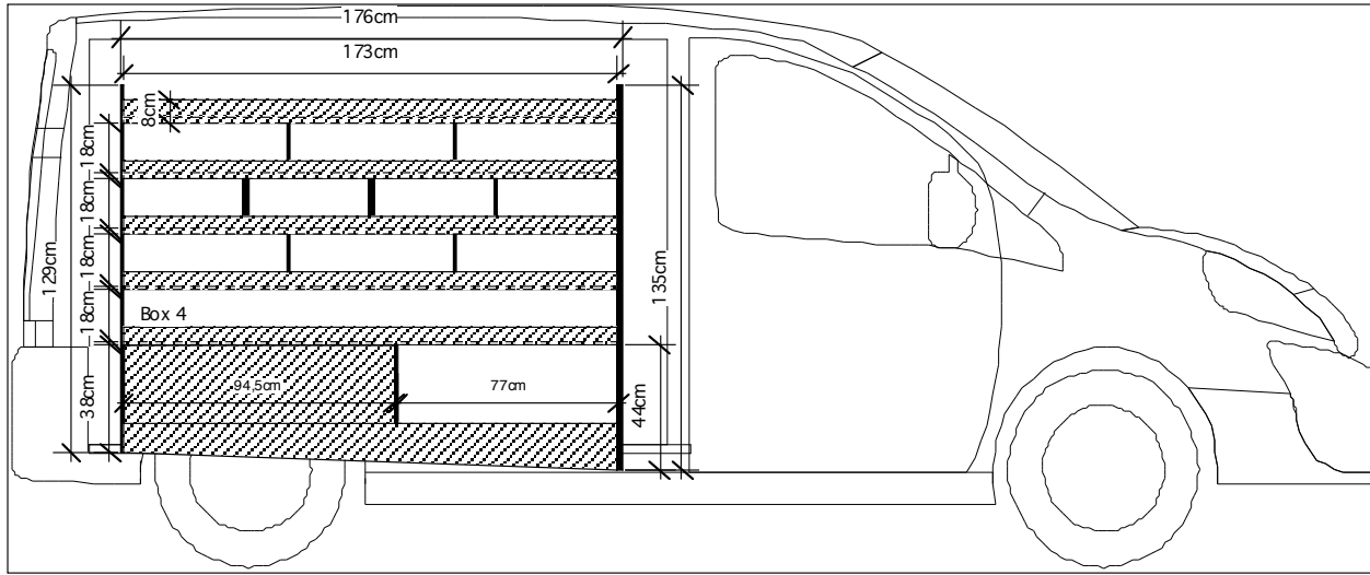
AGENCEMENTT EXPERT/JUMPY/SCUDO L1H1 (TRADE ADVANCE) VUE GAUCHE
