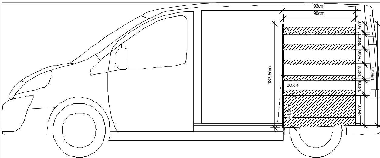
AGENCEMENTT EXPERT/JUMPY/SCUDO L1H1 (TRADE ADVANCE) VUE DROITE
