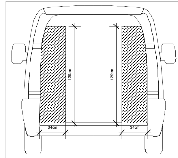
AGENCEMENTT EXPERT/JUMPY/SCUDO L1H1 (TRADE ADVANCE) VUE ARRIERE
